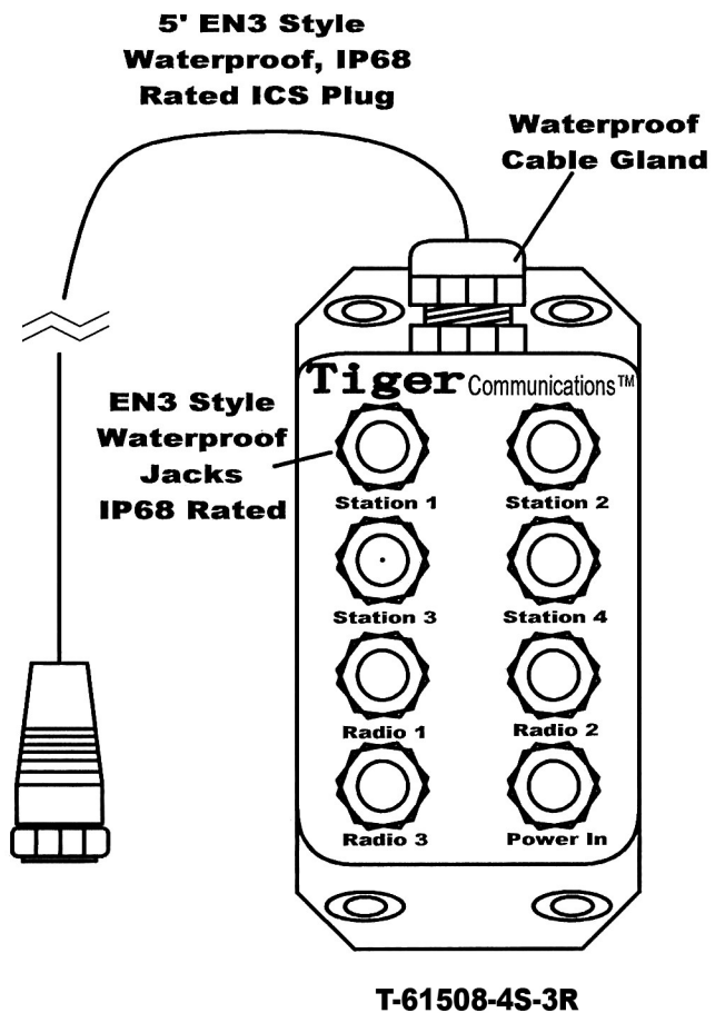
4 Station, 3 Radio Cable Junction Box
